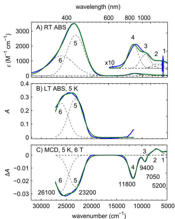
Figure 6. Optical spectra resolving six transitions in the near-IR and near-UV; bands 1–4 are copper based d \rightarrow d_{x^2-y^2} transitions, bands 5–6 are O(\text{TFE}) \rightarrow \text{Cu } d_{x^2-y^2} transitions. (A) Room temperature UV–vis and near-IR absorption spectrum of \text{Cu}^{\text{II}}\text{-O}(\text{TFE}) in DCM (from ref 21). (B) Electronic absorption of a thin film of \text{Cu}^{\text{II}}\text{-O}(\text{TFE}) collected simultaneously with MCD spectrum at 5 K and 0 T. (C) MCD spectrum of a thin film of \text{Cu}^{\text{II}}\text{-O}(\text{TFE}) acquired at 5 K and 6 T. Individual fitted Gaussian resolved bands are shown as dashed gray lines, the total fit in green, and experimental data in blue. The \lambda_{\text{max}} of transitions 1–6 are labeled in the MCD spectrum.
